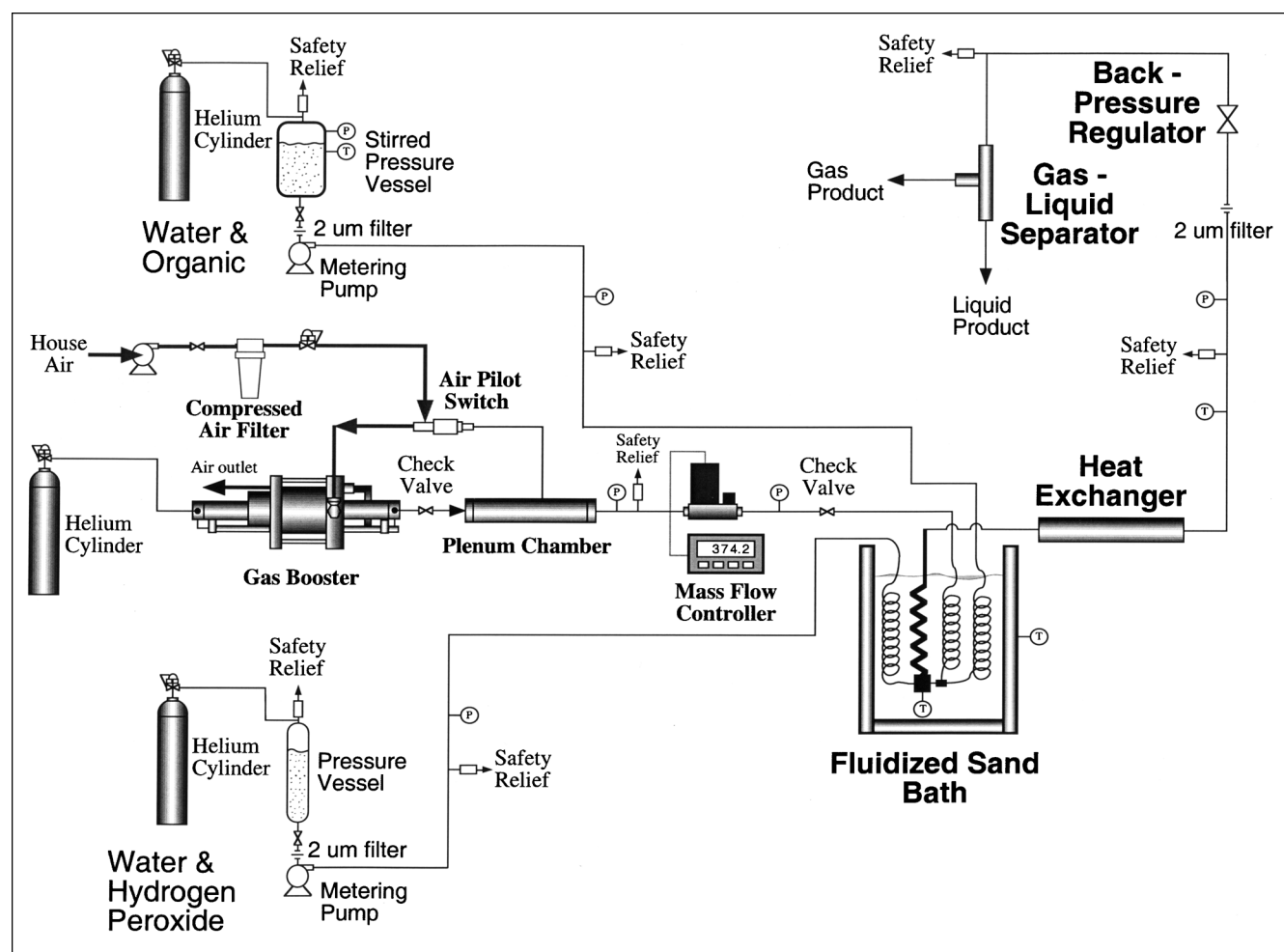
Figure 1. Experimental apparatus.
